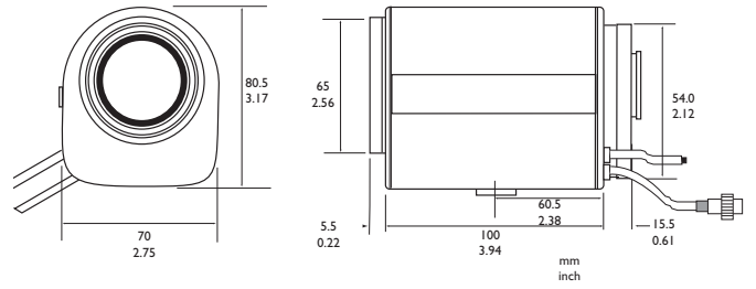
Dimensions LTC 3283/50
